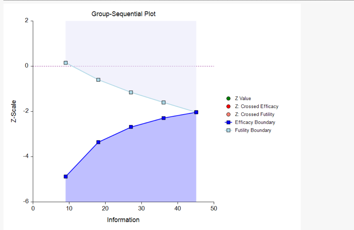
Group-Sequential Boundary Plot at Planning Stage (Stage 0)
